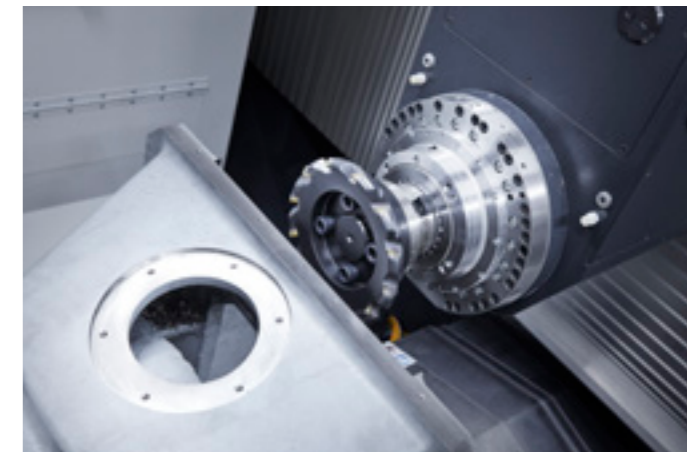
A WIDE RANGE OF ELECTROSPINDLES AVAILABLE The program offers a large variety of spindles available, to cover from high dynamics machinings to works on the hardest materials by high torque spindles.
